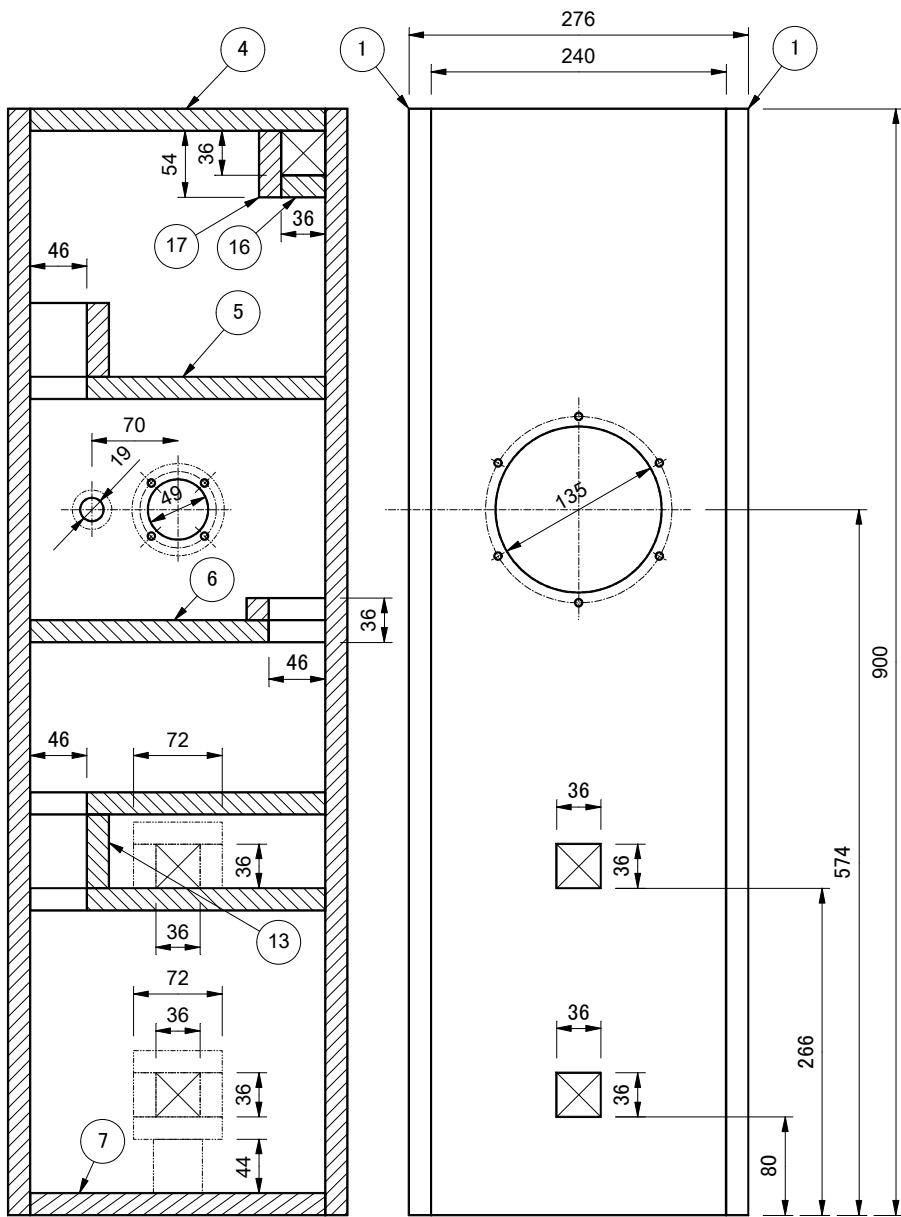
SECTION "ABCDEF"
