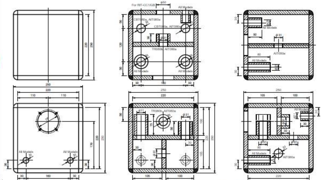
TR080b / AIT080a / CBT080a Assembly (Actual Drawing)
